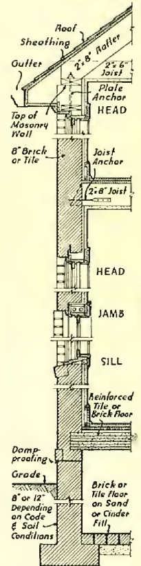
Wall Section
